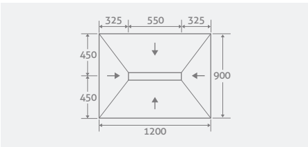
Four Falls 1200 x 900 x 30 37848 £868
