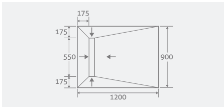
Four Falls 1200 x 900 x 30 37847 £868
