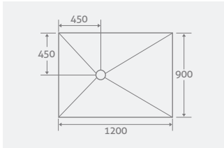
Offset Drain 1200 x 900 x 20 12854 £350
