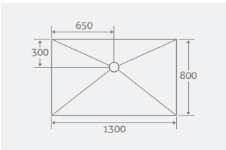
Offset Drain 1300 x 800 x 20 12856 £350
