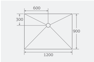
Offset Drain 1200 x 900 x 20 12855 £350
