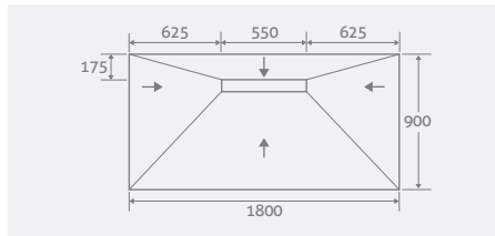
Four Falls 1800 x 900 x 30 37850 £977
